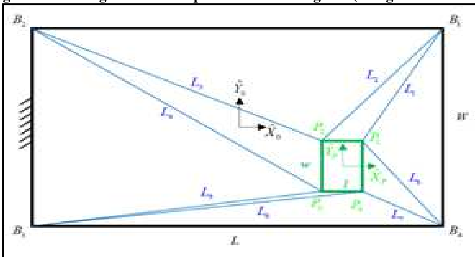
Figure No.2b: Top-View Kinematic Diagram(Design Candidate 3)
