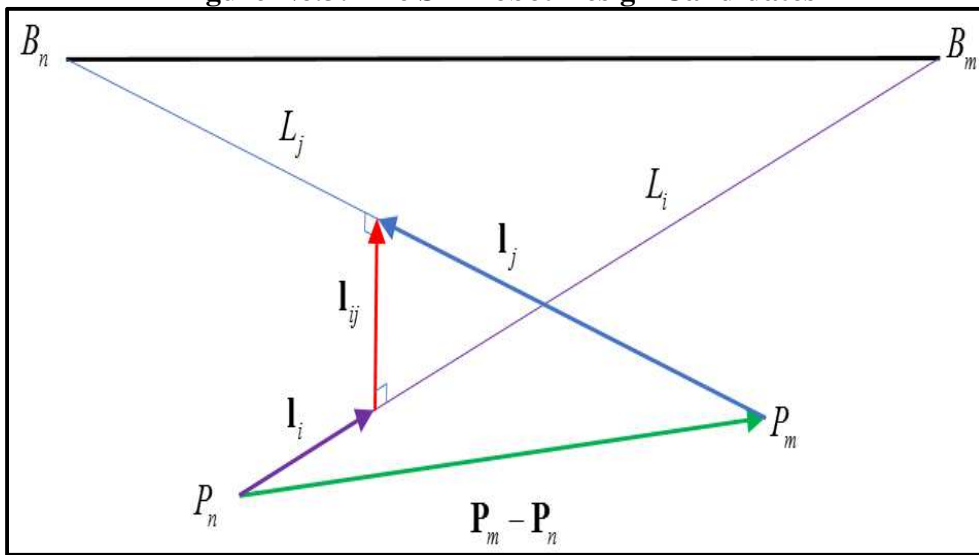
Figure No.4: Two-Cable Interference Diagram
