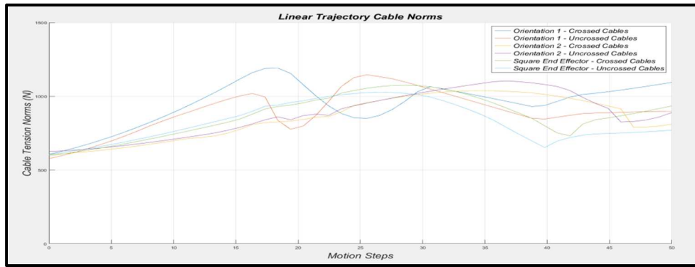
Figure No.8: Cable Tension Norms during Linear Trajectory for each Robot Design
