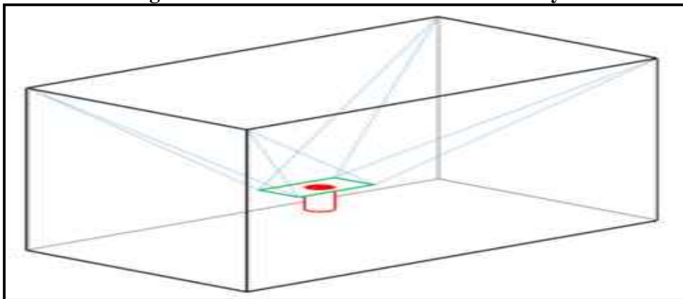
Figure No.2a: Eight-Cable-Suspended Robot Diagram (Design Candidate 1)
