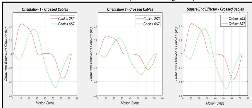
Figure No.11: Distances between Cables 2-3 and 6-7, Circular Trajectory cable interference occurs
