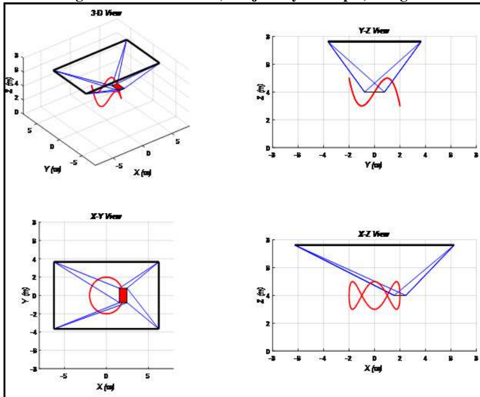
Figure No.7: Circular Trajectory Example, Design 3
