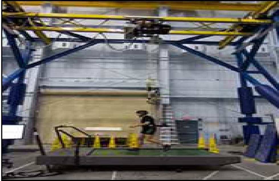
Figure No.1: NASA JSC ARGOS Laboratory
