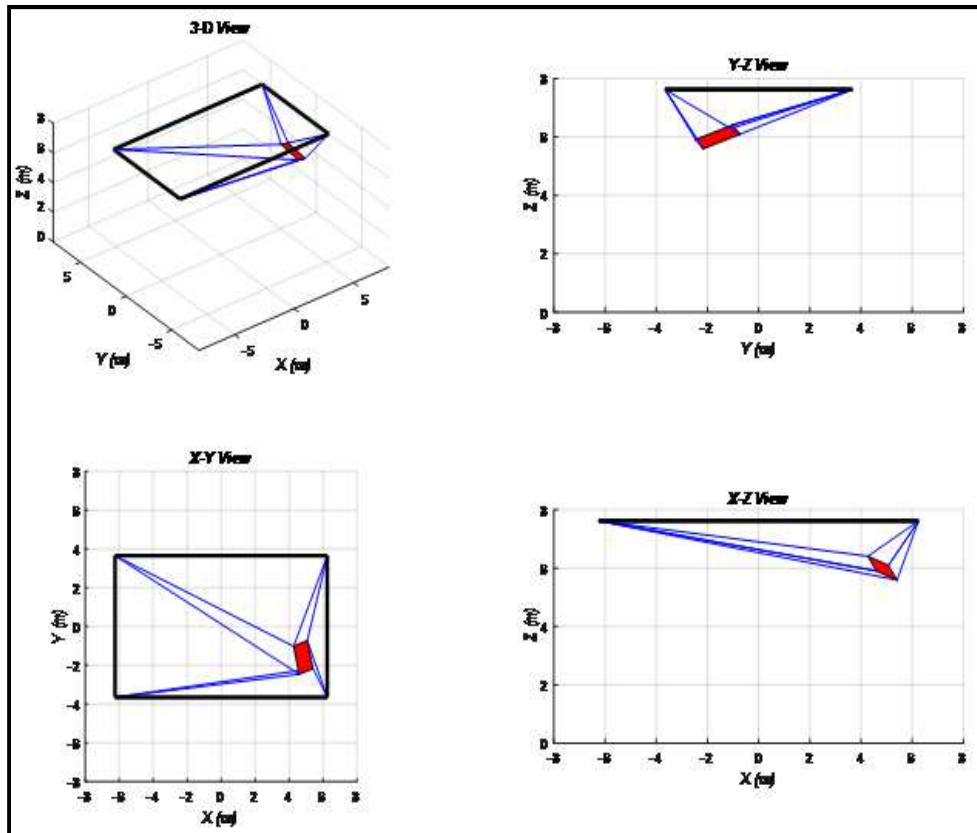
Figure No.6: Final Pose, Trajectory Example, Design 3
