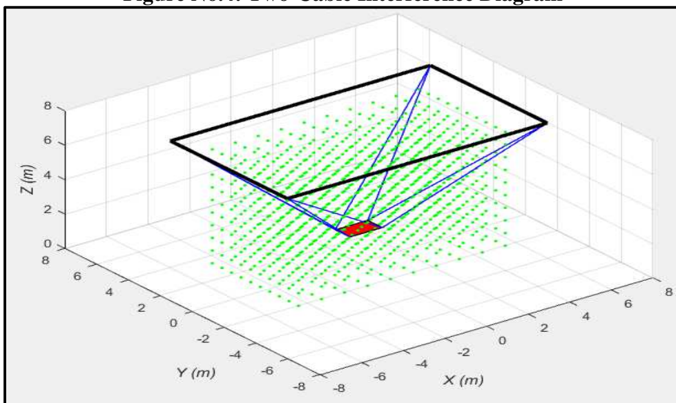
Figure No.5: All-Positive-Cable-Tension Workspace
