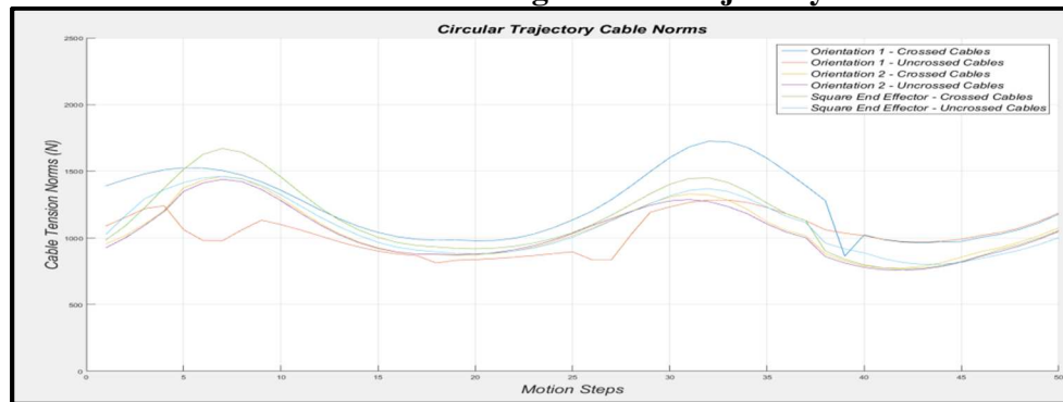
Figure No.9: Cable Tension Norms during Circular Trajectory for each Robot Design
