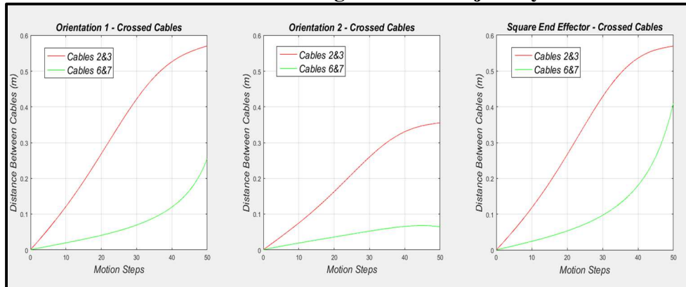
Figure No.10: Distances between Cables 2-3 and 6-7, Linear Trajectory no cable interference after start
